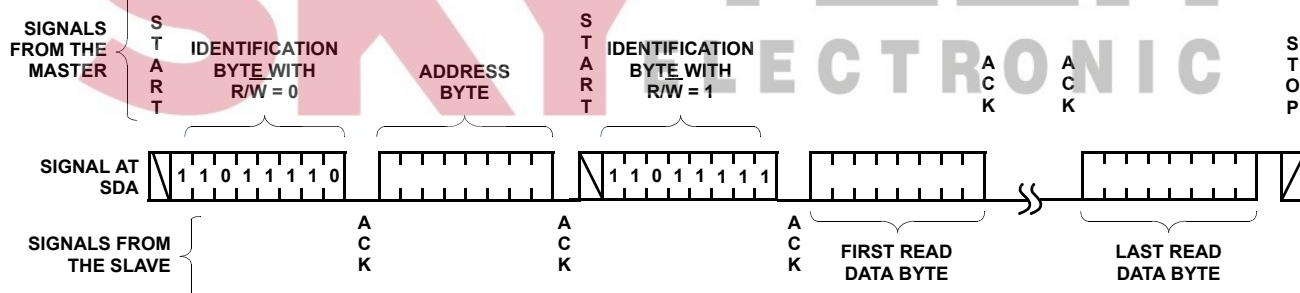
FIGURE 16. READ SEQUENCE
